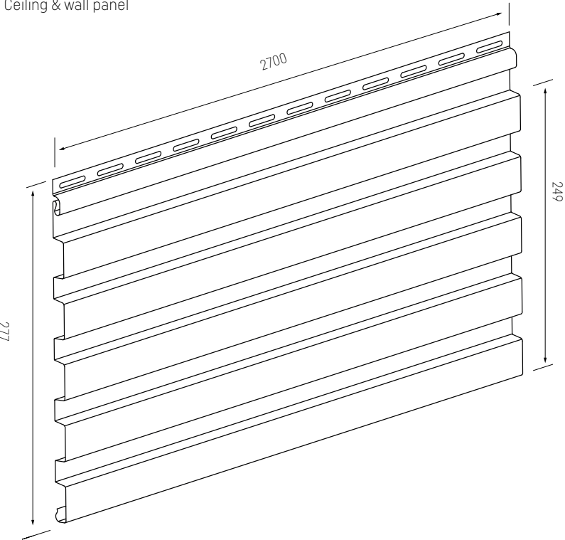
SV(P) 22 Ceiling & wall panel
