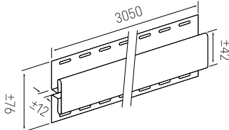
SV(P) 18 Joint trim
