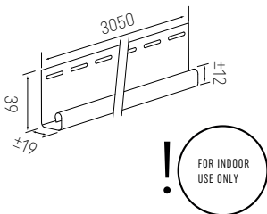
SV(P) 15.5 IN J-trim
